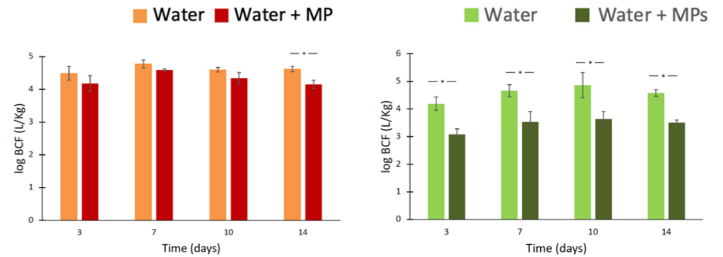
Figure 11. Effect of MPs on the bioconcentration of pesticides (Chlorpyrifos (left) and Hexachlorobenzene (right) in fish ( Danio rerio ), showing the presence of MPs lowered exposure.
