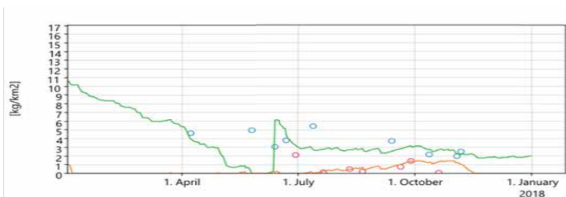
Figure 13. Model application to the Canadian case study. Upper panel shows the fit between modelled (red line) and observed (blue dots) river water discharges (driven in the model by an underlying hydrological module). The lower panel shows predicted (green and red lines) vs observed (blue and red dots, respectively) masses of MPs in the catchment soils over time. (green shows results for soils with applied sludge while red represents control soils).
