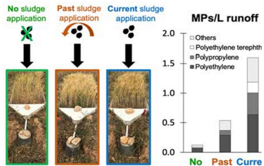
Figure 3 Experimental set-up with field plots and runoff analysis conducted in the Spanish case study
